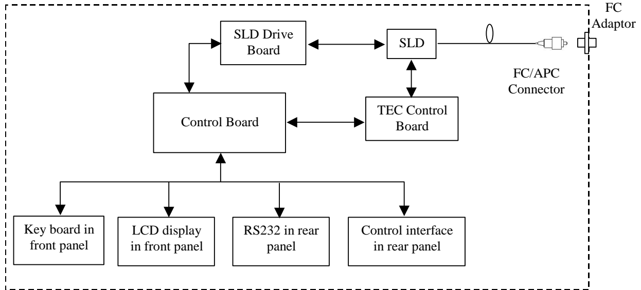
Figure 1 Configuration of IPSDM1311-xxxxx SLD light source desktop
