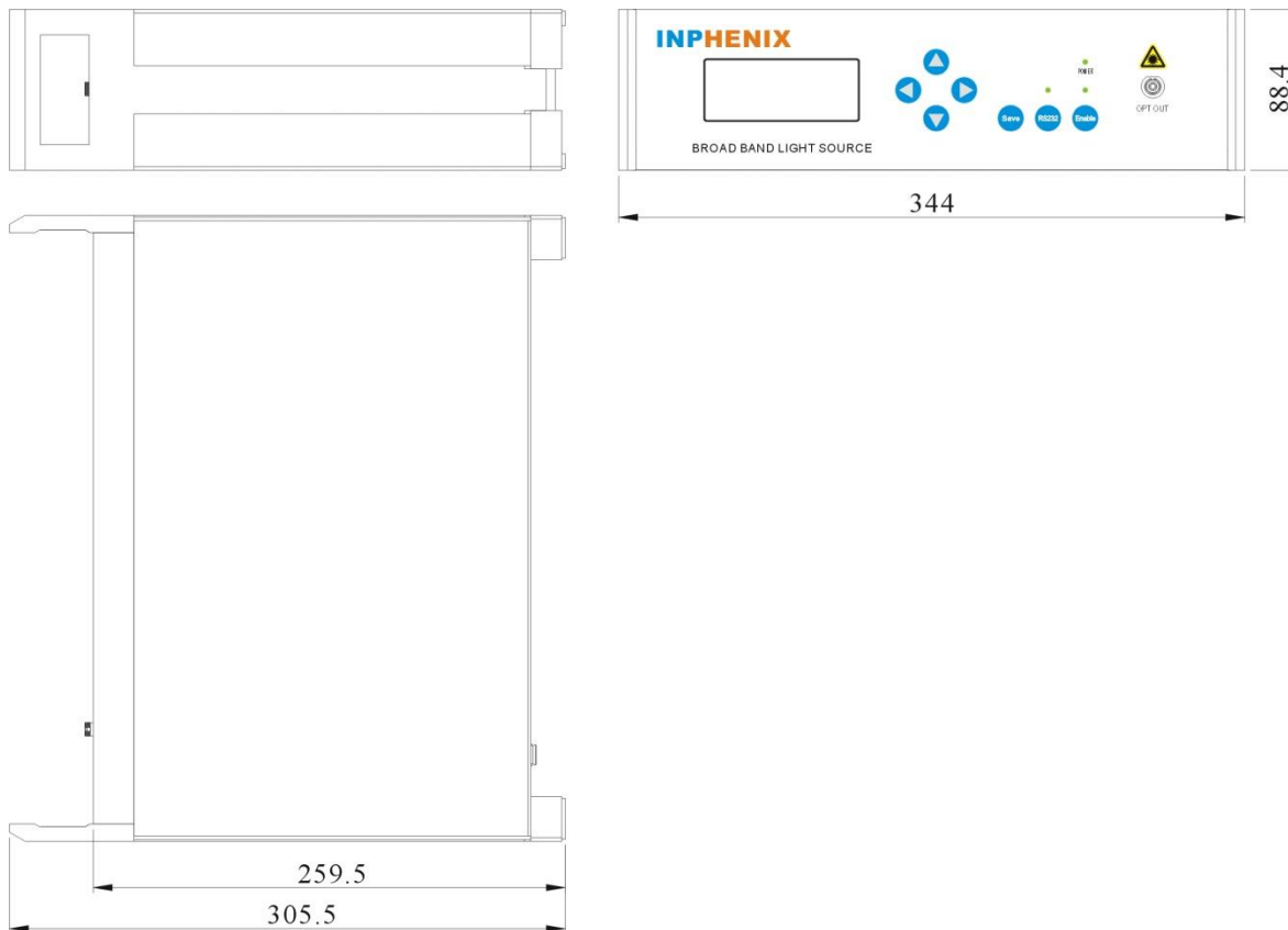
Figure 2 Mechanical drawing of IPSDM1311-xx×8 SLD light source desktop
